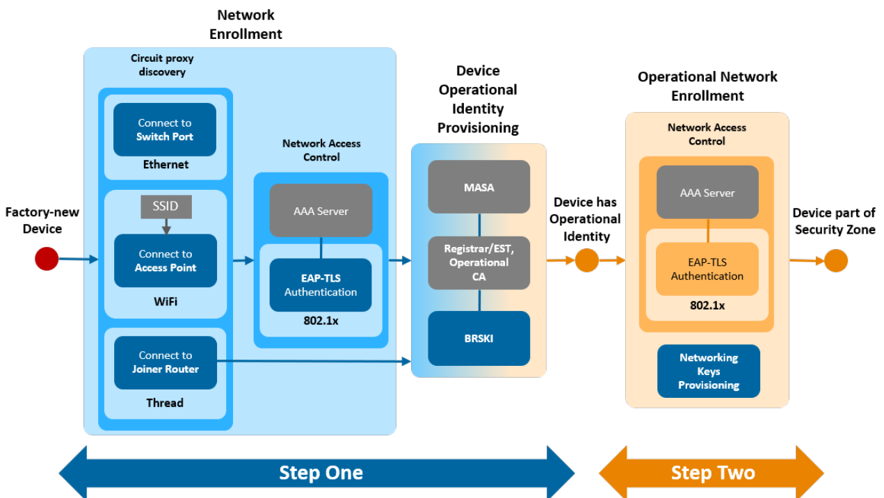
Figure 7: Device enrollment into a security zone
