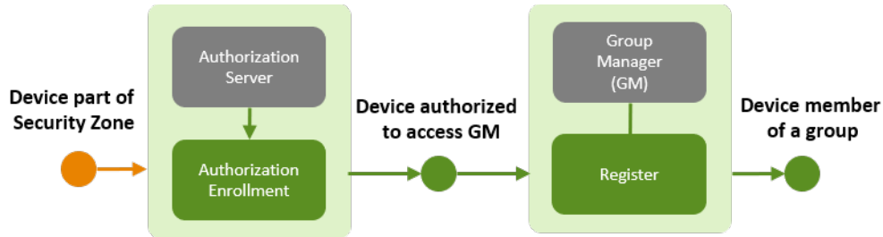
Figure 15: Multicast group establishment
