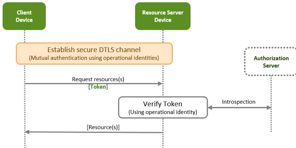
Figure 14: Resource request
