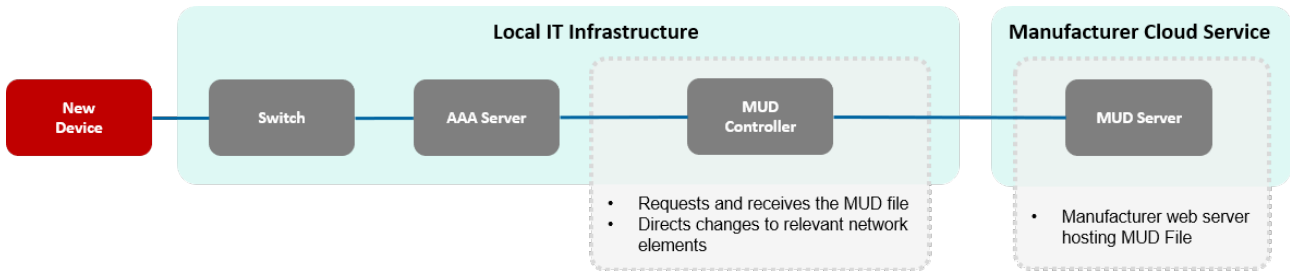
Figure 10: MUD Architecture
