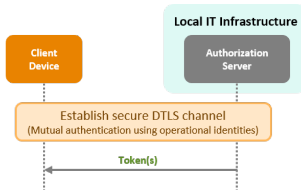
Figure 13: Authorization token enrollment
