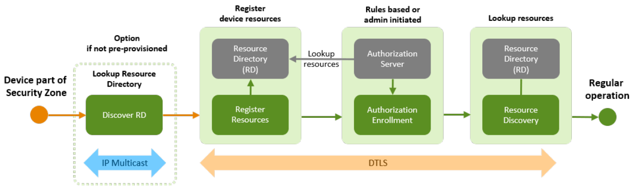
Figure 12: Authorization enrollment flow
