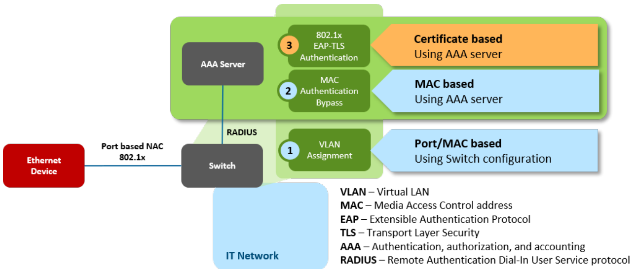
Figure 8: Network Access Control options for Ethernet devices
