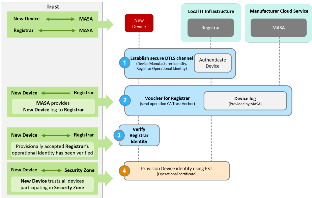
Figure 9: BRSKI identity provisioning process
